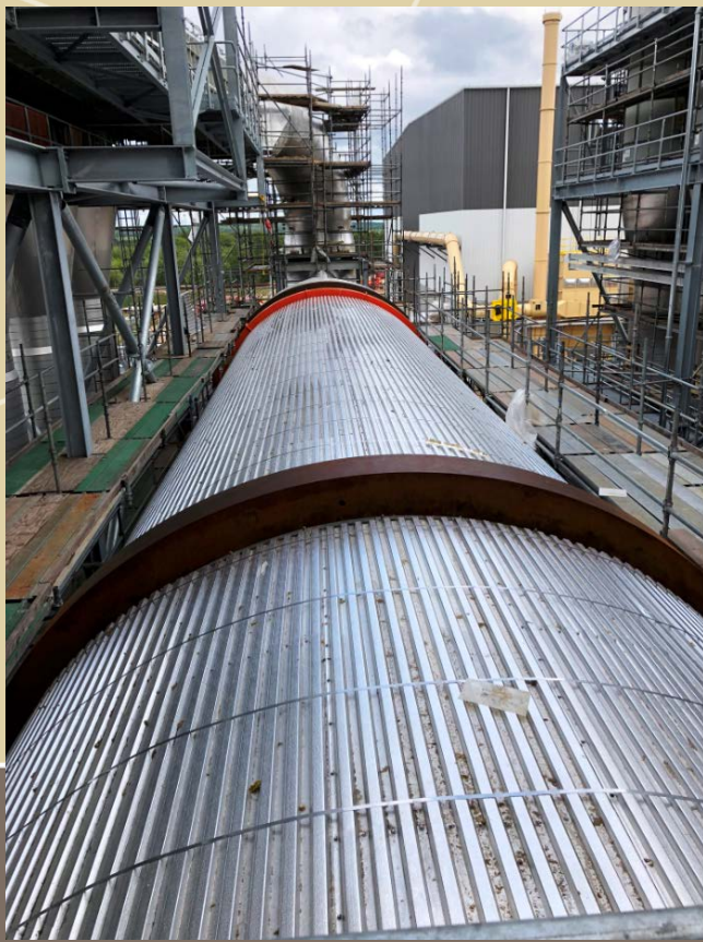
Dryer drum cladding – nearing completion
